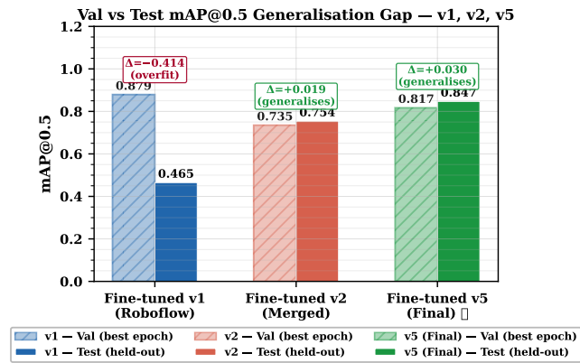
FIGURE 20. Validation-to-test mAP@0.5 gap across dataset versions. Takeaway: the 0.414-point v1 gap collapses to +0.030 at v5, consistent with dataset diversity (rather than architecture) driving generalisation.
