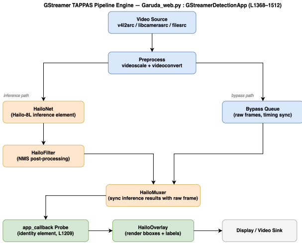
FIGURE 6. GStreamer TAPPAS pipeline topology. The fork-and-mux design lets the bypass queue hold the raw frame while HailoNet runs inference on the NPU, so the CPU touches each frame only at the identity callback probe – enabling the sustained 52.2 FPS reported in Section V-L.
