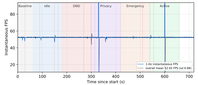
FIGURE 17. FPS-across-modes time series under full concurrent load (1 Hz probe, 720 s). Shaded regions mark the scheduled mode windows; vertical markers tag the injected load events: five real SMTP alerts, three encrypted clip-upload cycles over SSH (paramiko SFTP), three voice/chat queries, and a sustained MJPEG pull held for the full trace. Filtered mean 52.26 \pm 0.76 FPS (p50 52.16, p95 53.00, n = 709 ); per-window means span only a 0.3 FPS band across Baseline, Idle, DND, Privacy, Emergency, and Active, confirming that the slow SMTP and SSH channels never enter the inference budget.
