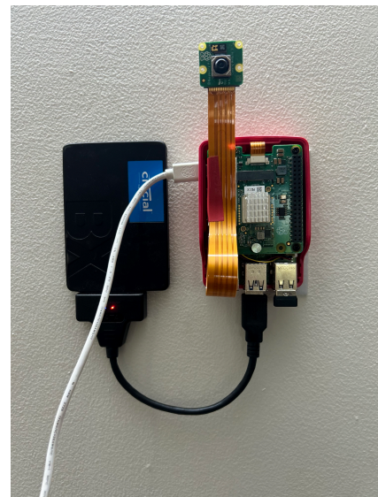
FIGURE 5. Deployed hardware — the exact rig on which every measurement in Section V was taken. Components visible in the photograph: Raspberry Pi 5 (16 GB, in a red active-cooled case), Hailo-8L AI HAT+ (13 TOPS), Raspberry Pi Camera Module v3 with its CSI-2 ribbon cable, and a 1 TB Crucial SATA SSD in a USB 3 enclosure. Total assembled BOM US$411; board power under deployed concurrent inference load is 5.89 \pm 1.43 W (Section V-J).
